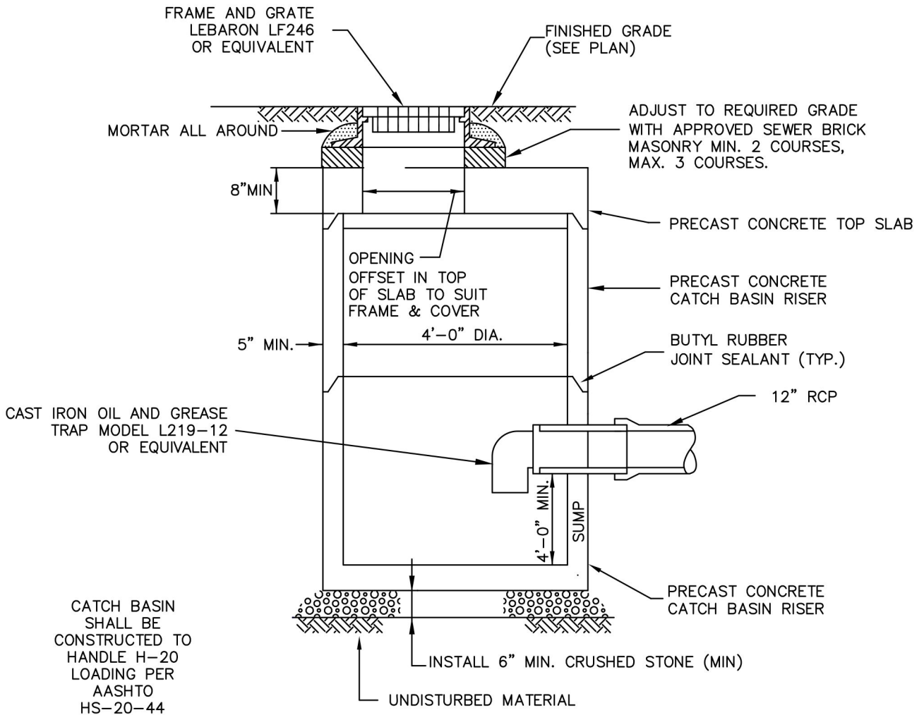
PRECAST CATCH BASIN DETAIL NOT TO SCALE
